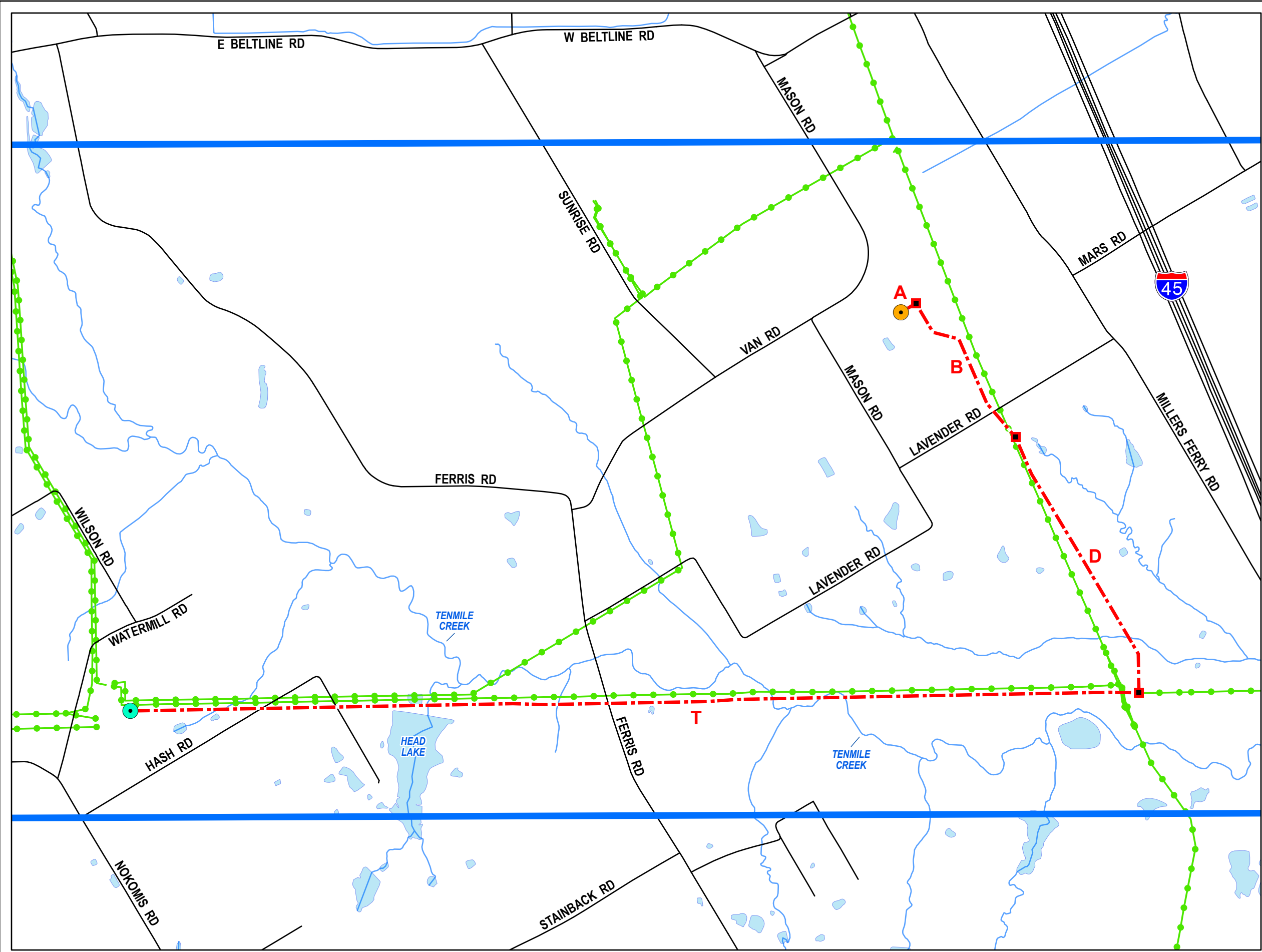
FIGURE 1 DETAILED ROUTE DESCRIPTION MAP WATERMILL SWITCH — WILMER SWITCH 345 KV TRANSMISSION LINE PROJECT
